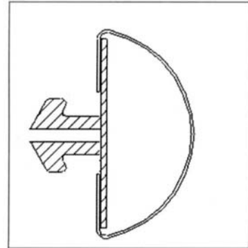
Universal Mounting
