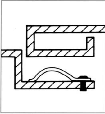
Rivet Mount
